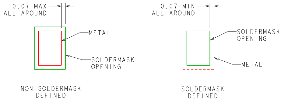
SOLDERMASK DETAILS
