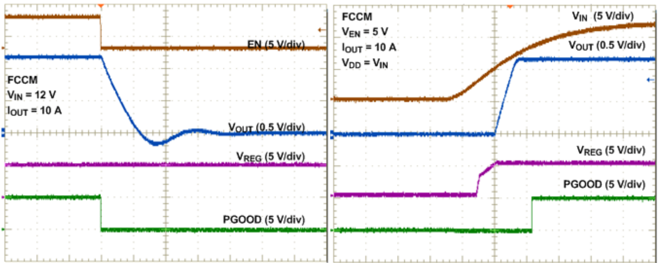
Time (40 \mu\text{s}/\text{div} ) Figure 29. Shutdown
