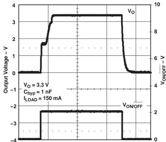
TURN-ON TIME
