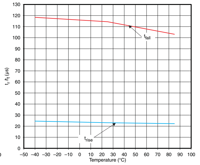
Figure 13. t_{rise}/t_{fall} vs Temperature ( V_{IN} = 3.3 V)
