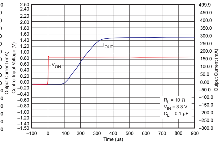
Figure 38. t_{ON} Response
