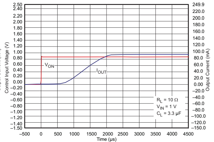
Figure 44. t_{ON} Response
