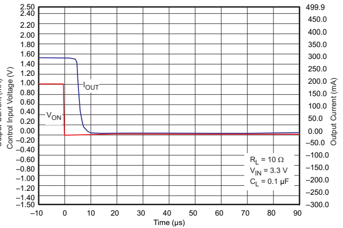
Figure 46. t_{OFF} Response
