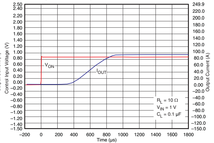
Figure 42. t_{ON} Response
