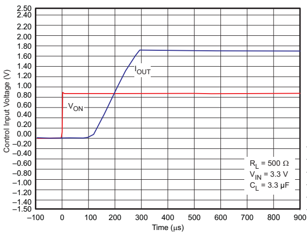
Figure 39. t_{ON} Response
