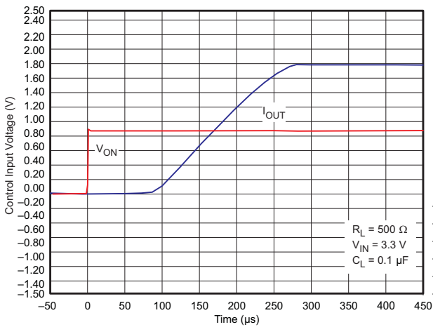
Figure 37. t_{ON} Response
