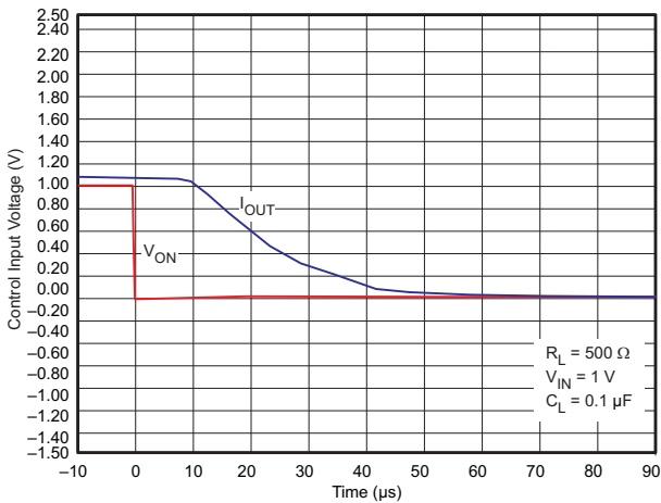
Figure 49. t_{OFF} Response
