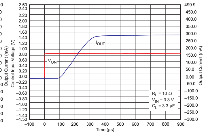
Figure 40. t_{ON} Response
