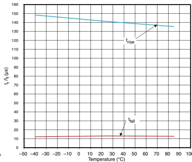
Figure 17. t rise /t fall vs Temperature (V IN = 3.3 V)
