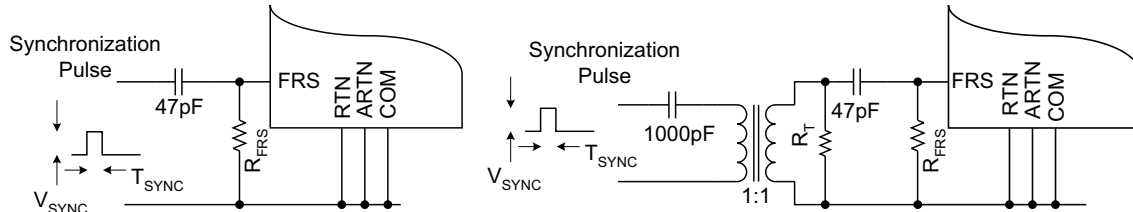
Figure 30. Synchronization
