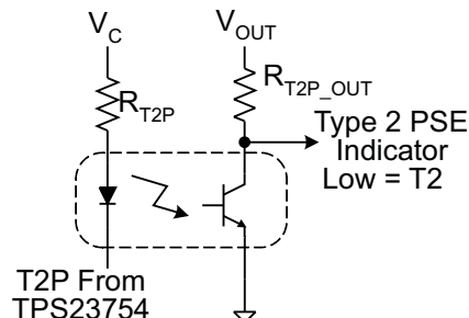
Figure 33. T2P Interface
