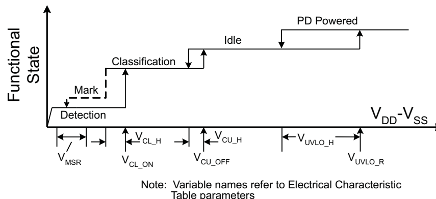
Figure 22. Threshold Voltages
