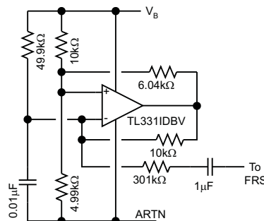
Figure 37. Frequency Dithering
