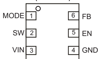
DRY PACKAGE (TOP VIEW)
