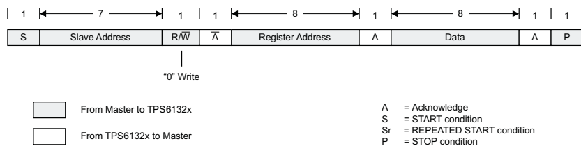
Figure 71. : "Write" Data Transfer Format in F/S-Mode
