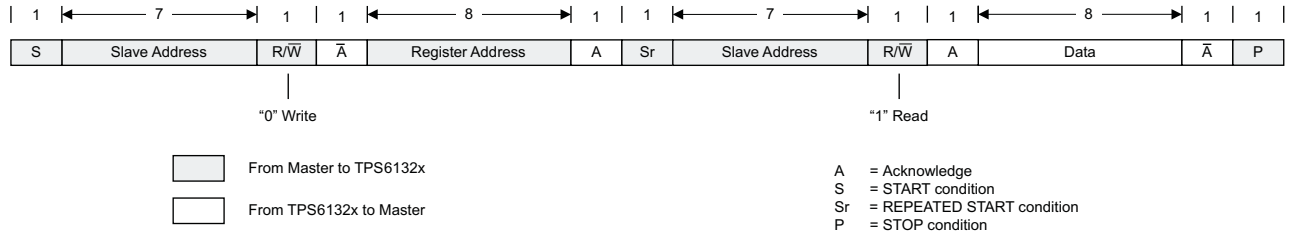
Figure 72. “Read” Data Transfer Format in F/S-Mode
