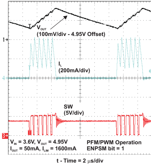
Figure 37. PFM OPERATION
