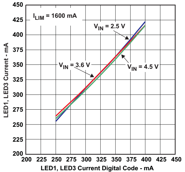
Figure 14. LED1, LED3 Current vs. LED1, LED3 Current Digital Code (HC_SEL=0)
