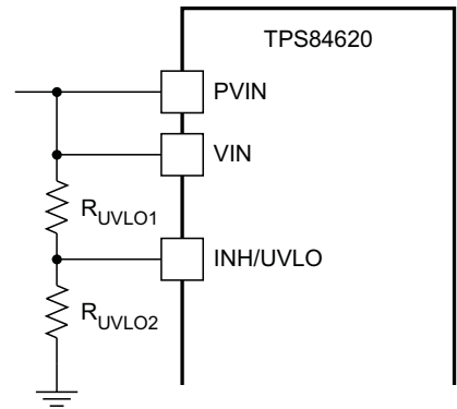
Figure 42. Adjustable VIN and PVIN Undervoltage Lockout
