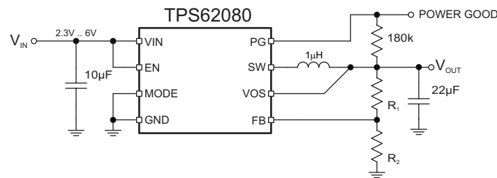
Figure 31. Typical Application Circuit for Adjustable Output Voltage Option
