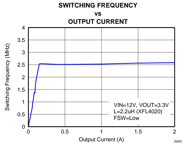
Figure 20. Switching Frequency
