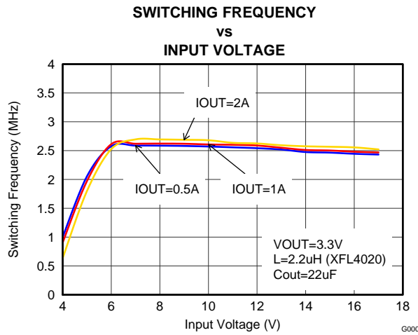
Figure 19. Switching Frequency
