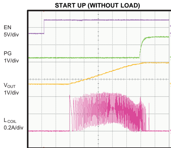
t - 20 \mu s/div Figure 17.
