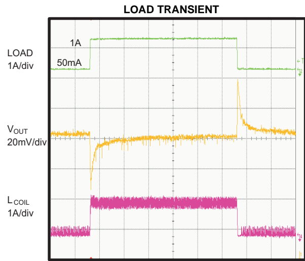
t - 50µs/div Figure 14.
