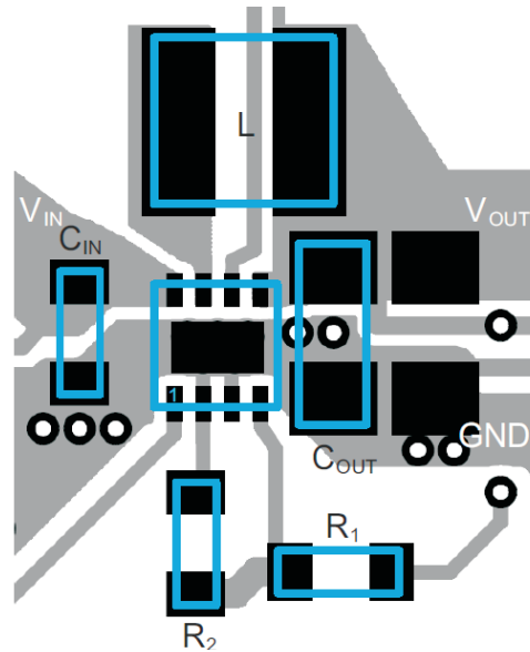
Figure 19. PCB Layout Suggestion
