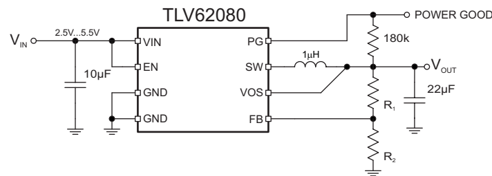
Figure 18. Typical Application Circuit
