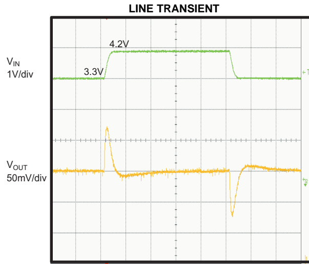
t - 100 \mu s/div Figure 15.
