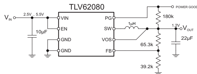
Figure 20. 1.2V Output Voltage Application
