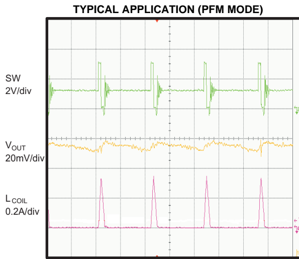
t - 2µs/div Figure 13.
