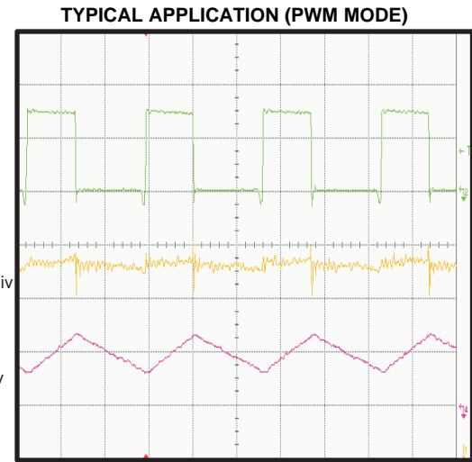
t - 200ns/div Figure 12.
