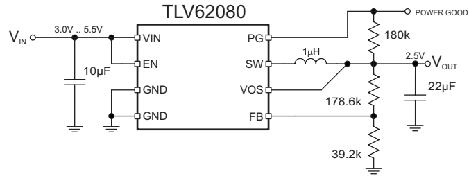
Figure 21. 2.5V Output Voltage Application
