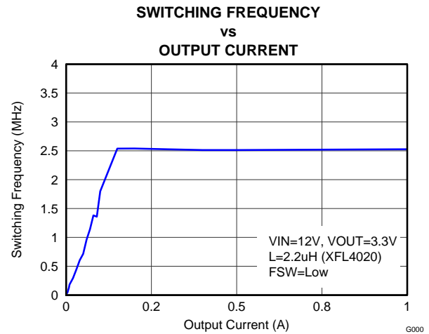
Figure 20. Switching Frequency
