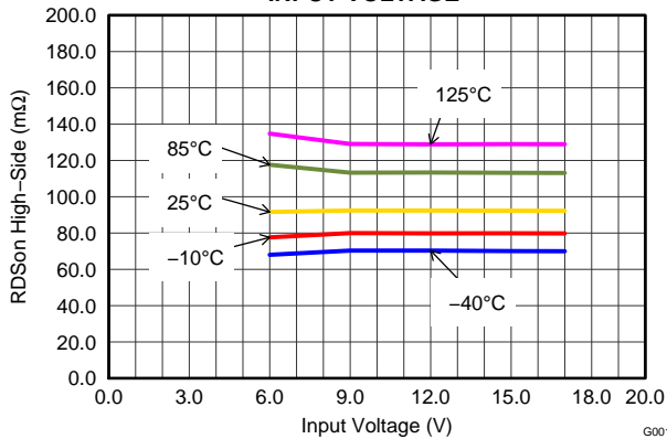
Figure 23. High-Side Switch Resistance
