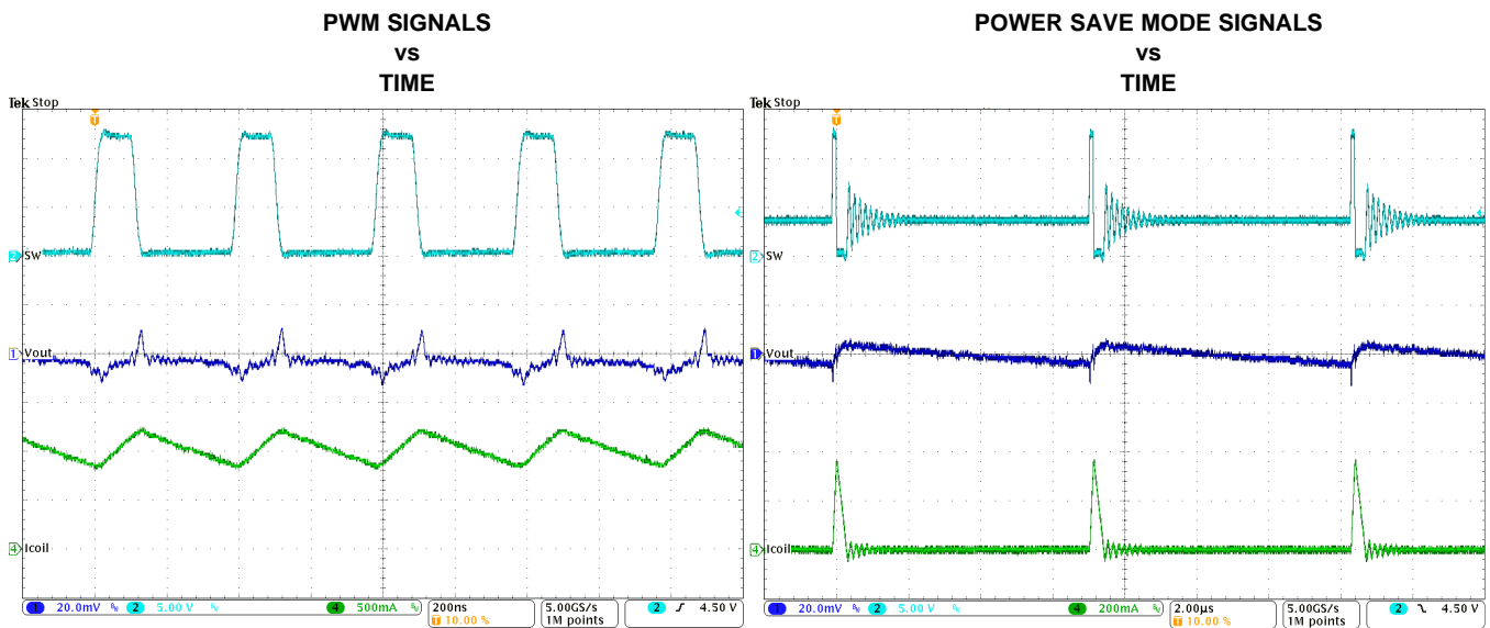
Figure 35. Typical Operation in PWM Mode (I OUT =1A)
