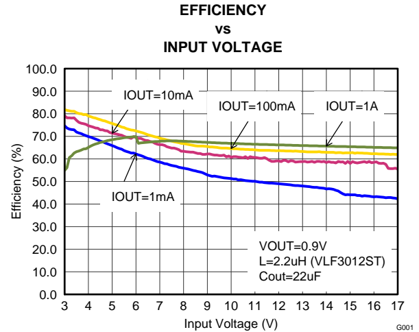
Figure 12. Vout=0.9V
