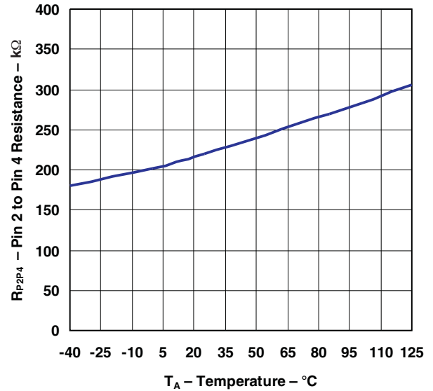
DIVIDER RESISTANCE VS TEMPERATURE
