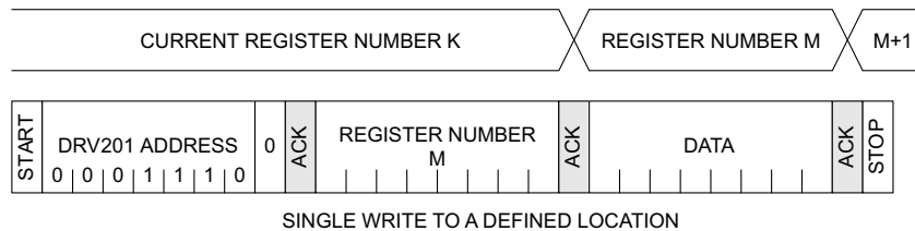
Figure 7. Single Write
