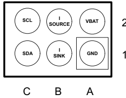
NanoFree YMB PACKAGE (BOTTOM VIEW)
