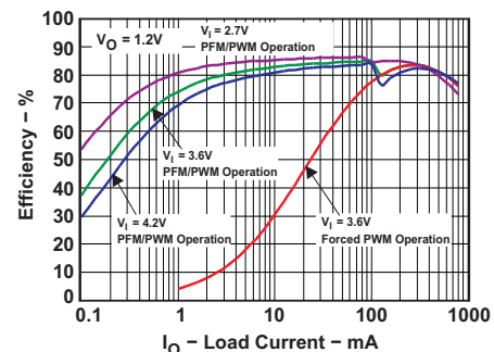
Figure 2. Efficiency vs Load Control
