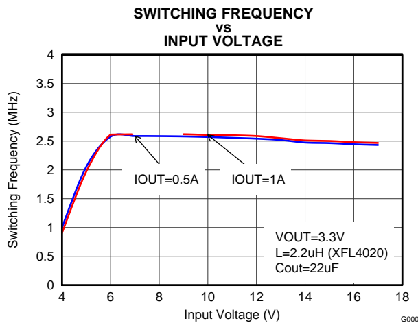
Figure 18. Switching Frequency
