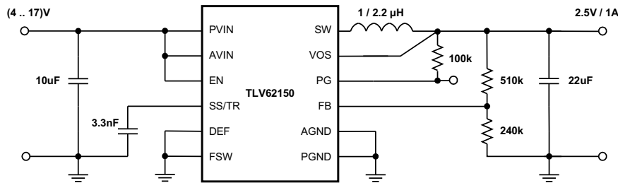
Figure 43. 2.5V/1A Power Supply
