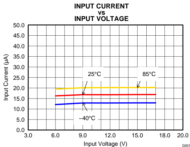
Figure 20. Quiescent Current
