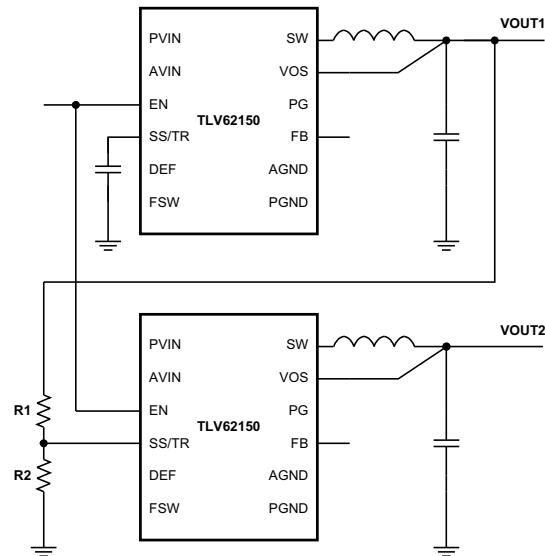
Figure 37. Sequence for Ratiometric and Simultaneous Startup
