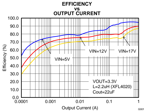
Figure 10. Efficiency with 2.5MHz, Vout=3.3V
