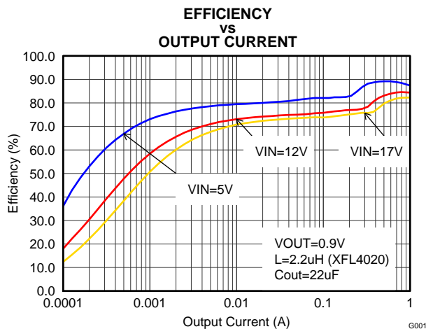
Figure 14. Efficiency with 1.25MHz, Vout=0.9V
