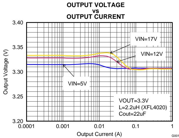
Figure 16. Output Voltage Accuracy (Load Regulation)
