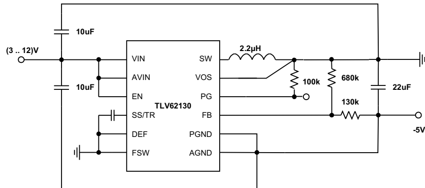
Figure 42. -5V Inverting Power Supply
