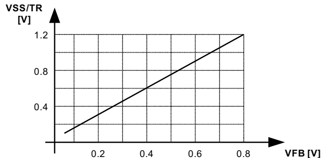
Figure 38. Voltage Tracking Relationship
