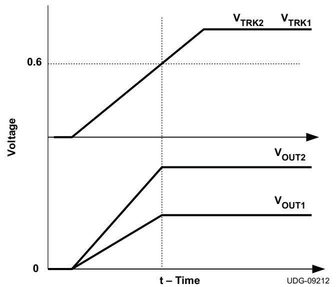
Figure 29. Ratiometric Voltage-Tracking Schematic Figure 30. Ratiometric Voltage-Tracking Waveform
