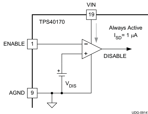
Figure 16. TPS40170-Q1 ENABLE Functional Block
