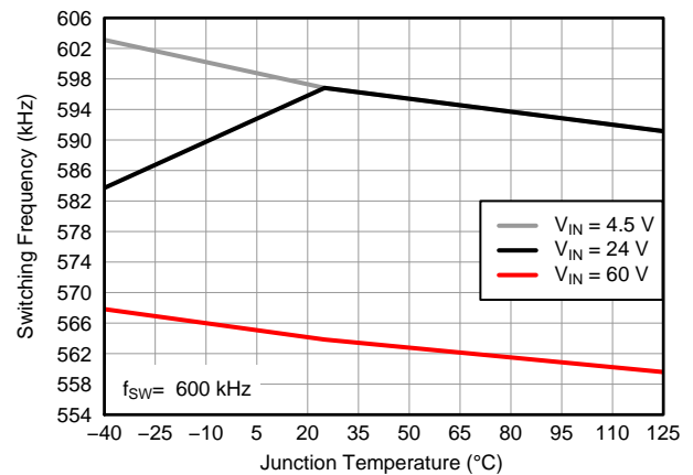
Figure 4. Switching Frequency vs Junction Temperature (f sw = 600 kHz)
