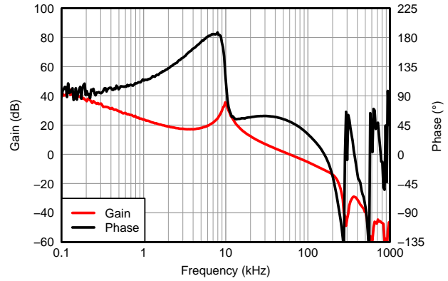
Figure 36. Loop Response
