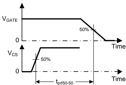
Figure 3. Time Delay from V_{CS} to V_{GATE}
