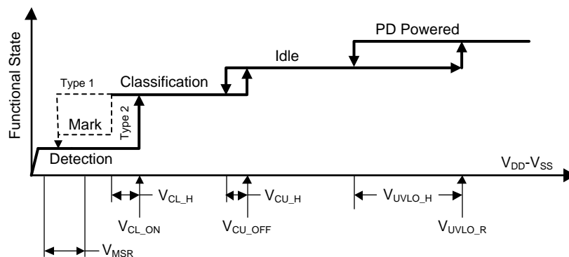
Figure 21. Threshold Voltages
