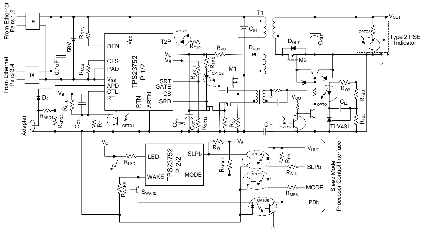
Figure 29. TPS23752 Application Circuit
