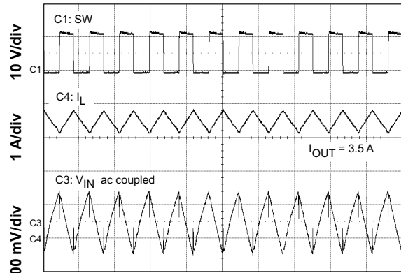
Time = 2 μs/div
