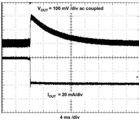
Figure 47. Unload Transient
