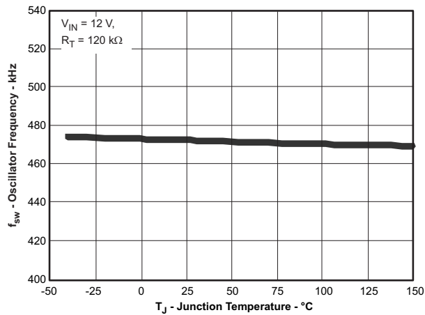
Figure 5. Frequency vs Temperature
