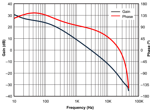
Figure 43. Frequency Response
