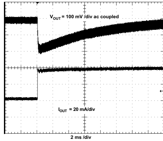
Figure 46. Load Transient
