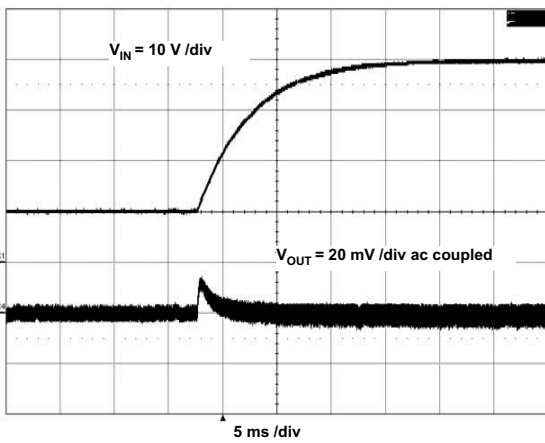
Figure 29. Line Transient
