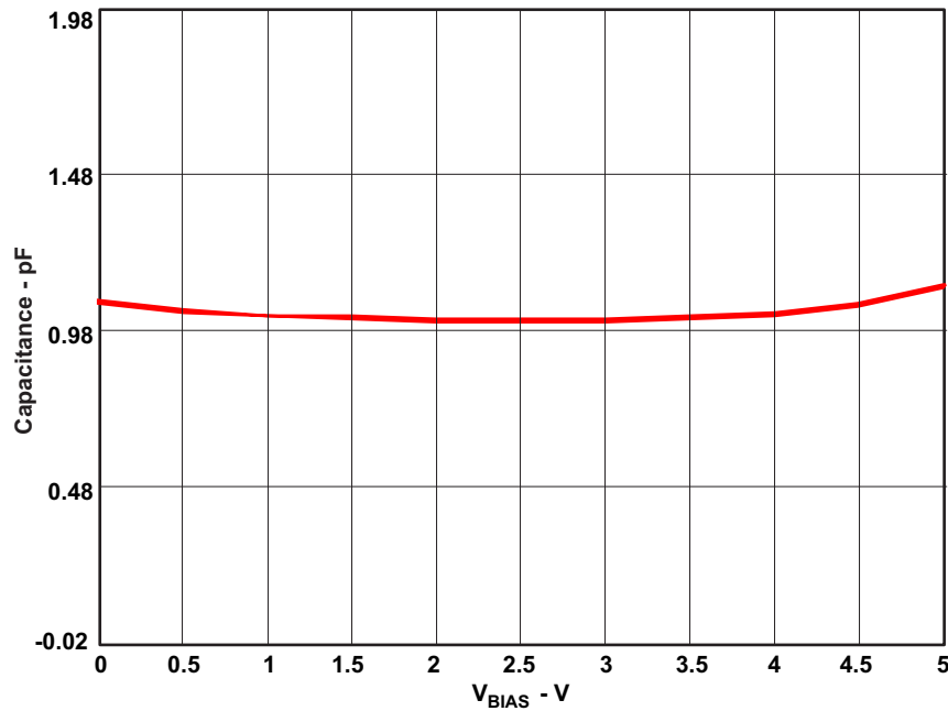
Figure 4. Pin Capacitance
