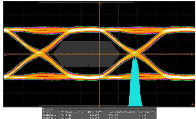
Figure 14. Eye diagram using EVM with TPD13S523 for the TMD5 Lines at 1080p, 340MHz pixel clock, 3.4Gbps
