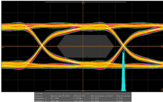
Figure 13. Eye diagram using EVM without TPD13S523 for the TMD5 Lines at 1080p, 340MHz pixel clock, 3.4Gbps
