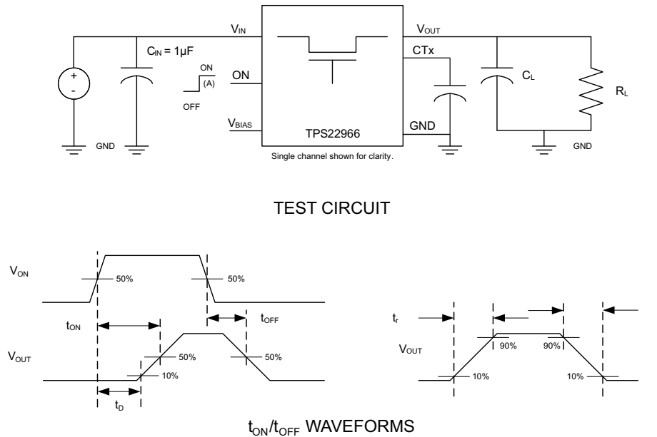
(A) Rise and fall times of the control signal is 100ns.
