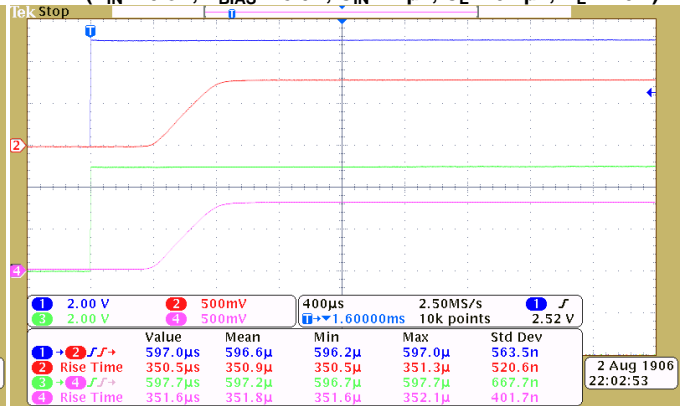
TURN-ON RESPONSE TIME ( V_{IN} = 5.0\text{V} , V_{BIAS} = 5.0\text{V} , C_{IN} = 1\mu\text{F} , C_L = 0.1\mu\text{F} , R_L = 10\Omega )
