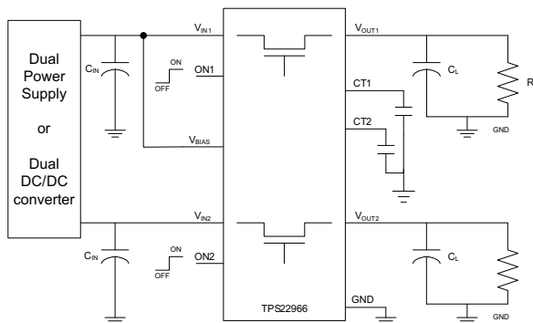
Figure 1. Typical Application
