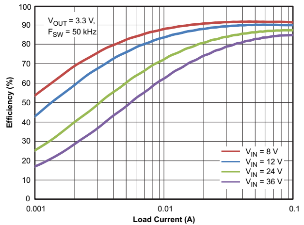
Figure 42. Efficiency vs Load Current
