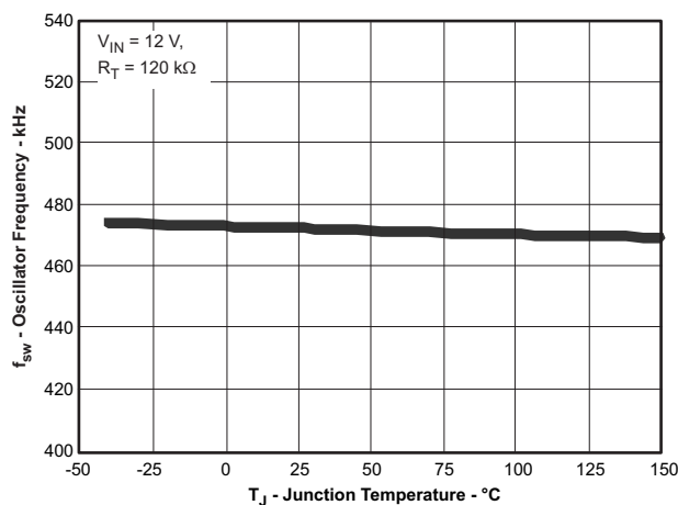
Figure 5. Frequency versus Temperature
