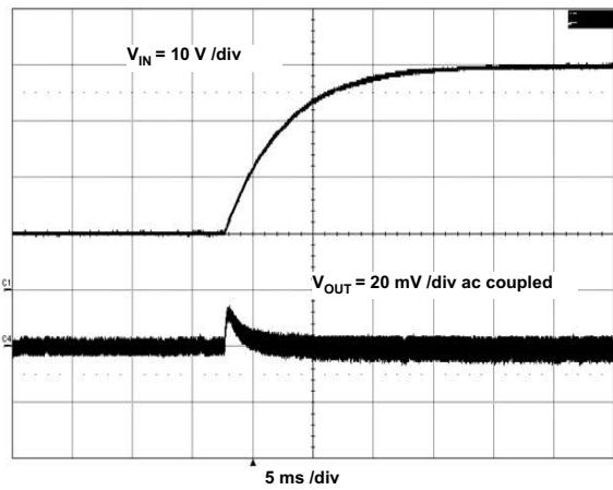
Figure 29. Line Transient
