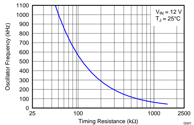
Figure 6. Frequency versus R_T/CLK Resistance
