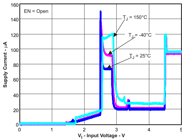
Figure 15. Supply Current (VIN pin) versus Input Voltage (0 V to VSTART), EN Pin Open
