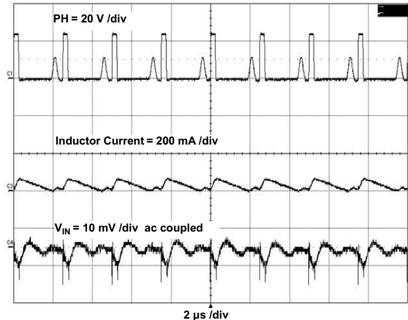
Figure 32. Input Ripple in DCM
