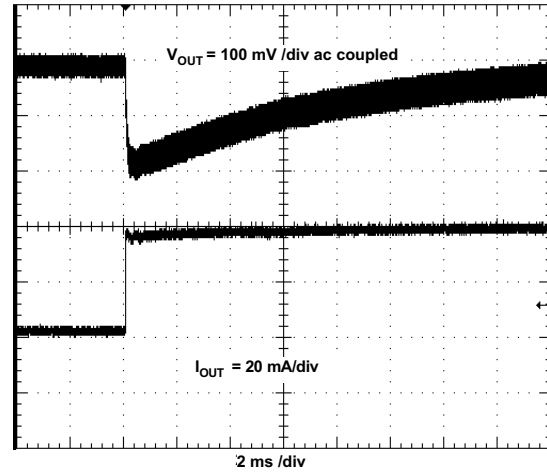
Figure 46. Load Transient
