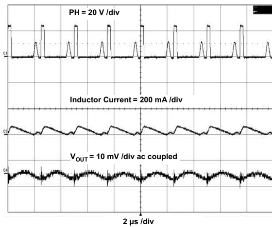
Figure 35. Output Ripple in DCM
