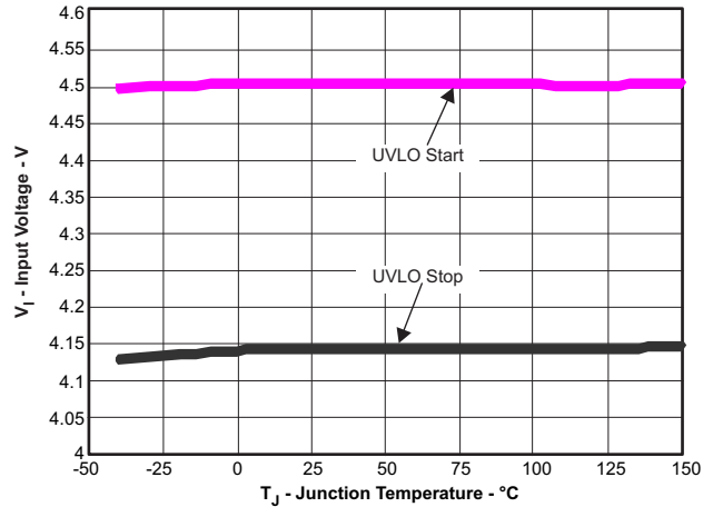
Figure 10. Input Voltage (UVLO) versus Temperature
