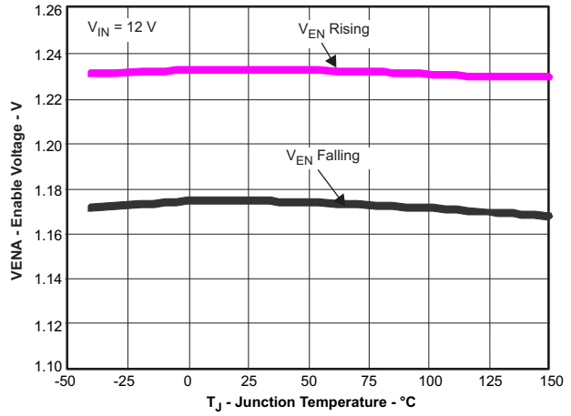
Figure 8. Enable-Pin Voltage versus Temperature
