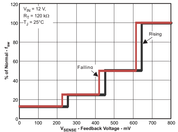
Figure 4. Frequency versus V_{SENSE} Voltage
