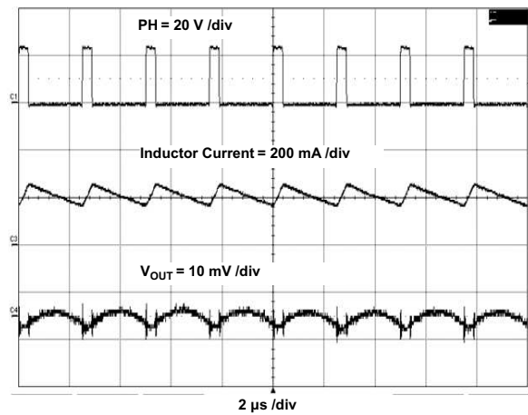
Figure 36. Output Ripple in CCM
