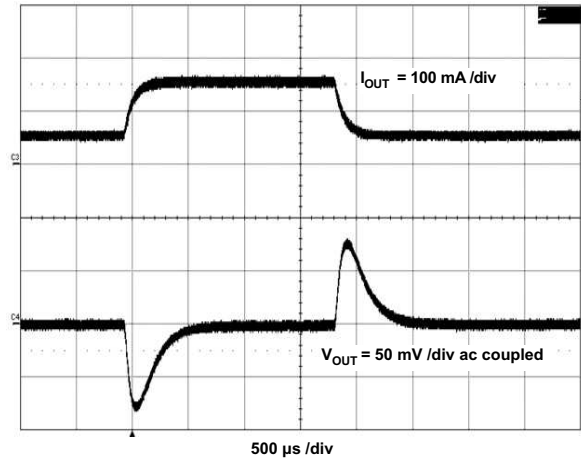
Figure 28. Load Transient
