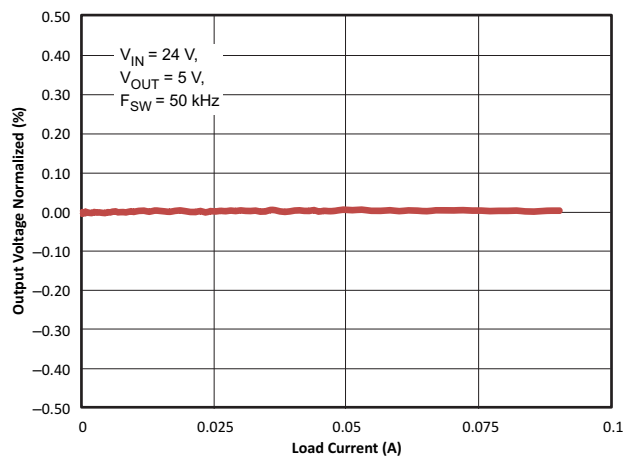
Figure 44. Output Voltage Normalized vs Load Current
