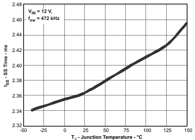
Figure 16. Slow-Start Time versus Temperature
