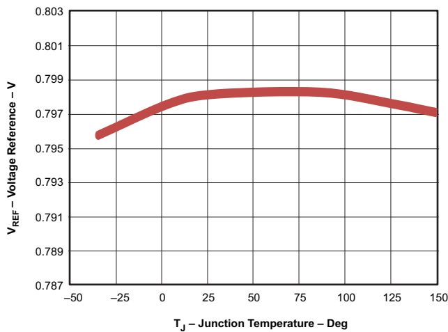
Figure 3. V_{REF} Voltage versus Temperature
