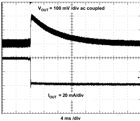
Figure 47. Unload Transient
