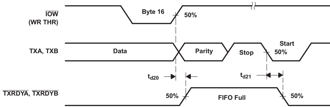
Figure 20. Trceiver Ready ( \overline{\text{TXRDY}} ) Waveforms, FCR0 = 0 and FCR3 = 1 (Mode 1)
