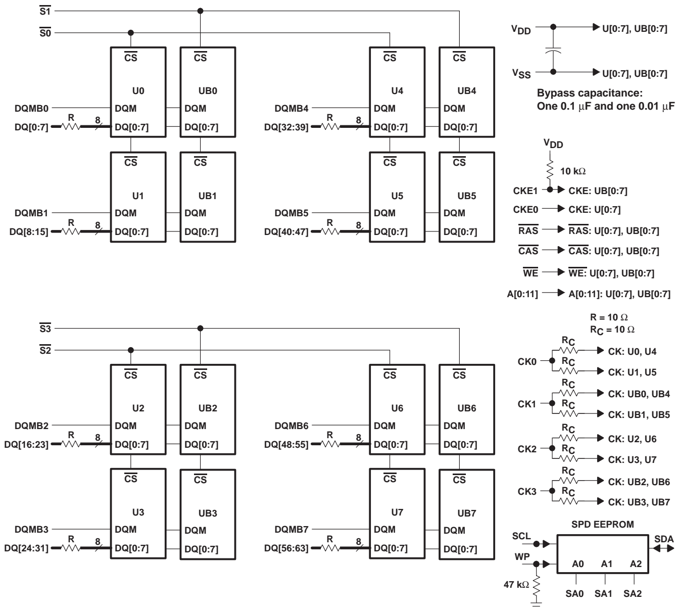
functional block diagram for the TM4CN64EFH
