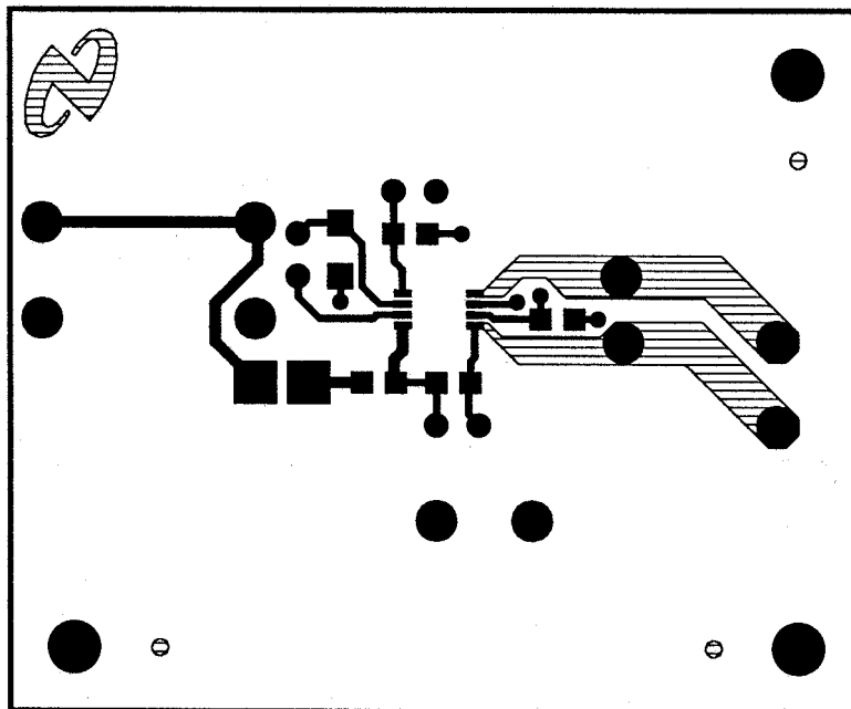
Figure 46. Top Layer
