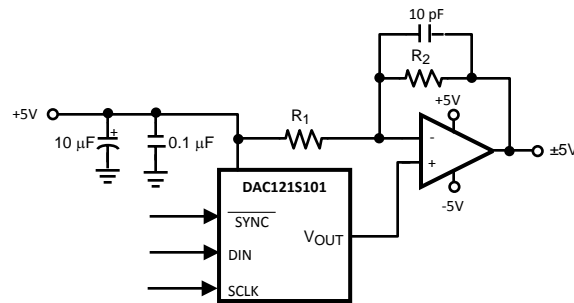
Figure 45. Bipolar Operation
