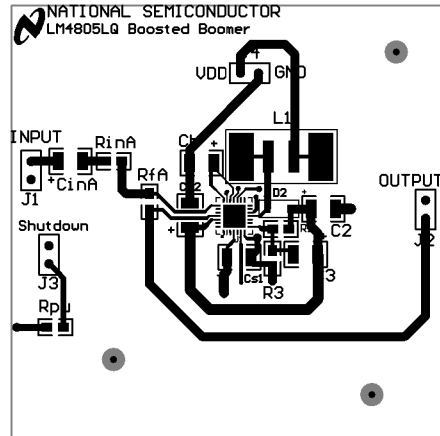
Figure 46. Silkscreen
