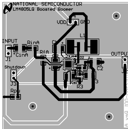
Figure 44. Composite Layer
