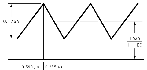
Figure 42. 10μH Inductor Current 5V - 12V Boost (LM4805)
