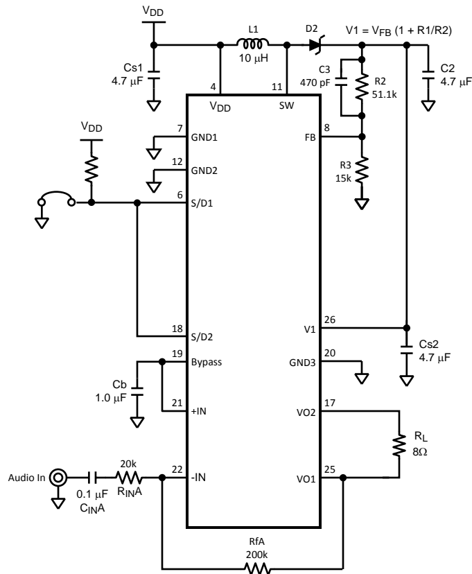
Figure 43. Demo Board Reference Schematic
