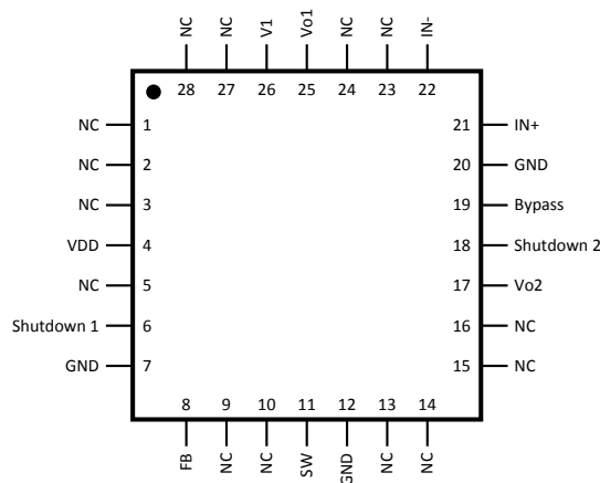
Figure 1. LM4805LQ (5x5) (Top View) See Package Number NJB0028A
