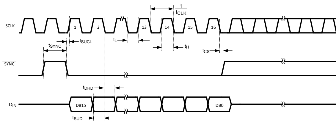
Figure 4. DAC101S101 Timing
