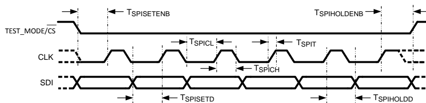
Figure 12. SPI Timing
