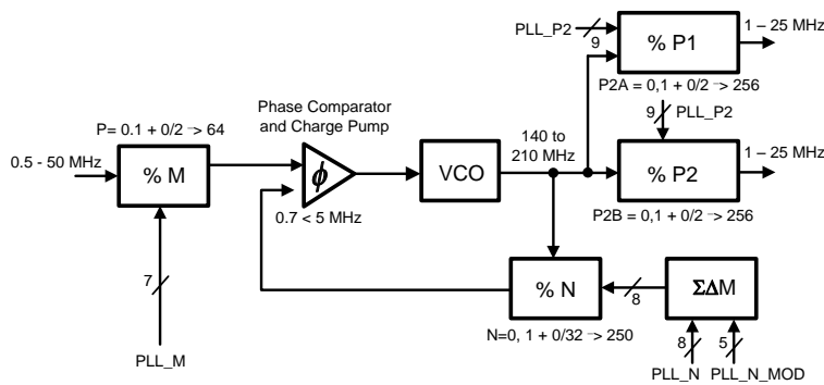
Figure 55. PLL1 Loop
