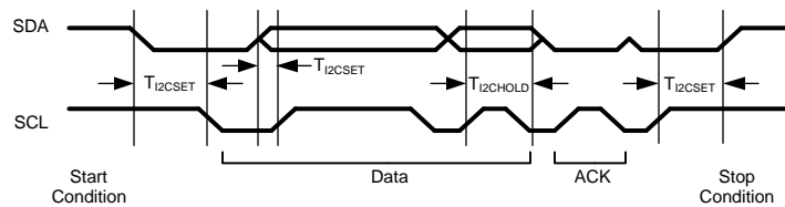
Figure 6. Two Wire Mode Write Bus
