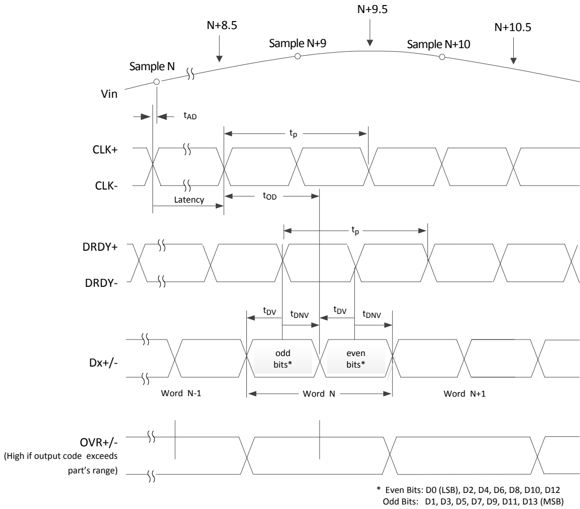
Figure 1. Output Timing
