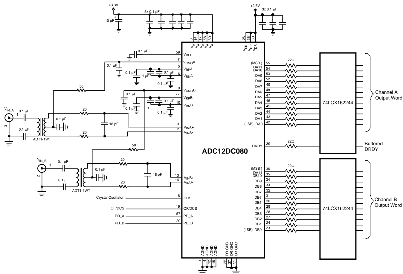
Figure 21. Application Circuit
