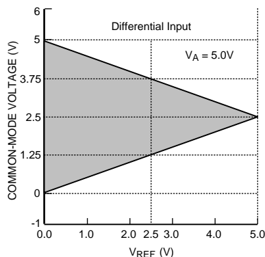
Figure 40. V_{CM} range for Differential Input operation
