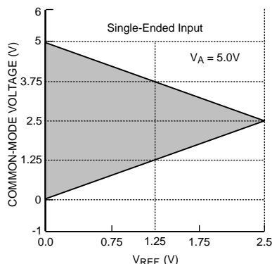
Figure 41. V_{CM} range for single-ended operation
