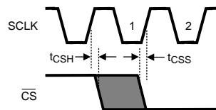
Figure 6. Valid \overline{\text{CS}} Assertion Times
