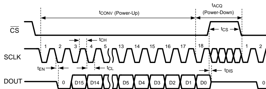
Figure 46. ADC161S626 Single Conversion Timing Diagram
