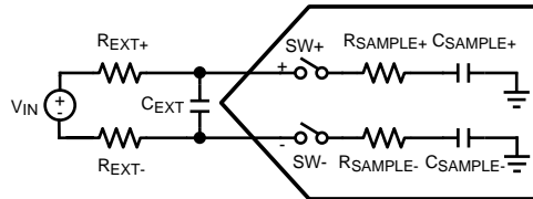
Figure 45. ADC Input Capacitors
