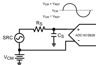
Figure 39. Single-Ended Input
