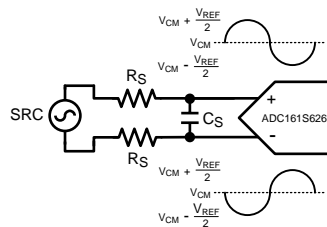
Figure 38. Differential Input
