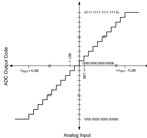
Figure 37. ADC Transfer Curve
