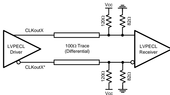
Figure 9-13. Differential LVPECL Operation, DC Coupling, Thevenin Equivalent
