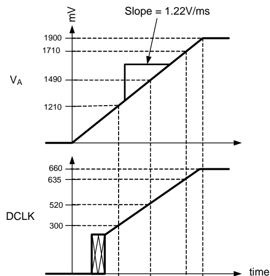
Figure 6-14. Supply and DCLK Ramping
