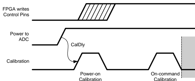
Figure 6-13. Power-on with Control Pins set by FPGA post Power-on Cal
