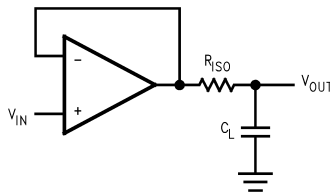
Figure 41. Isolating Capacitive Load
