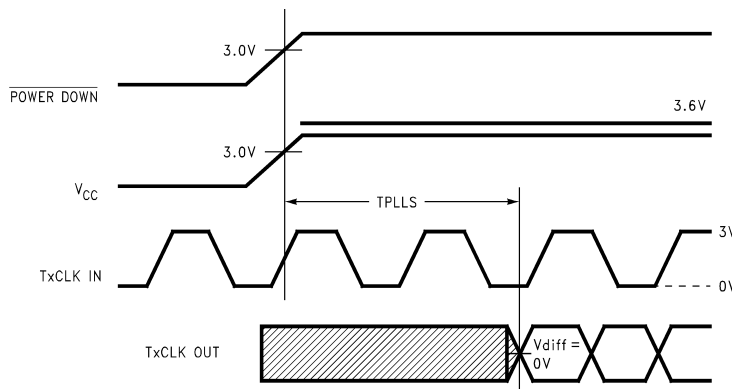
Figure 9. DS90C363A/DS90CF363A (Transmitter) Phase Lock Loop Set Time
