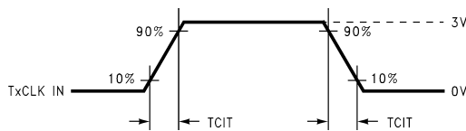
Figure 6. DS90C363A/DS90CF363A (Transmitter) Input Clock Transition Time
