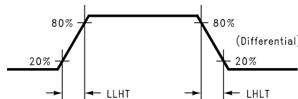
Figure 5. DS90C363A/DS90CF363A (Transmitter) LVDS Transition Times
