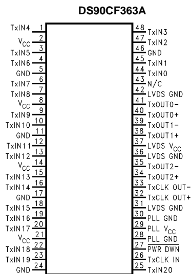
Figure 16. 48 Pin TSSOP - See Package Number DGG
