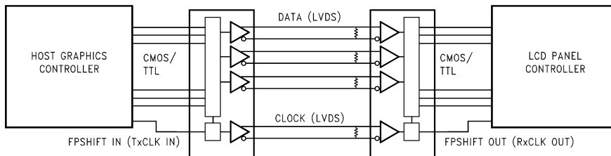
Figure 17. Typical Application
