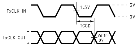
Figure 8. DS90C363A/DS90CF363A (Transmitter) Clock In to Clock Out Delay (Falling Edge Strobe)
