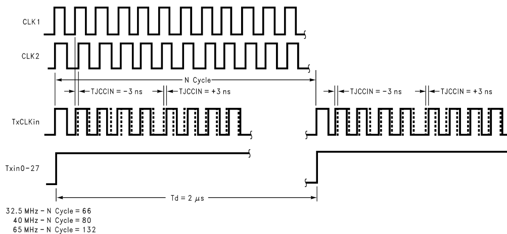
Figure 14. Timing diagram of the Input cycle-to-cycle clock jitter
