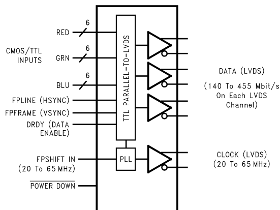
Figure 1. DS90C363A/DS90CF363A
