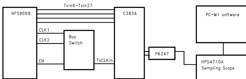
Figure 13. TJCC Test Setup
