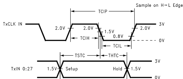
Figure 7. DS90C363A/DS90CF363A (Transmitter) Setup/Hold and High/Low Times (Falling Edge Strobe)
