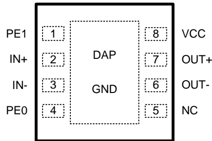
WSON Package
