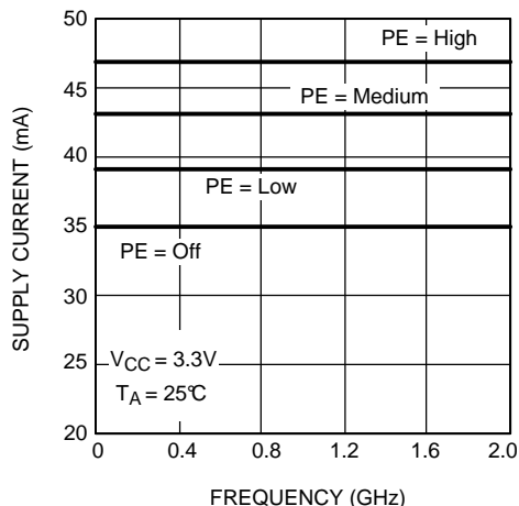
Figure 13. Power Supply Current as a Function of Frequency
