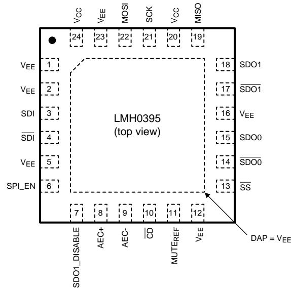
Figure 2. SPI Mode / SPI_EN = V CC , 24-Pin WQFN Package See Package Number RTW0024A
