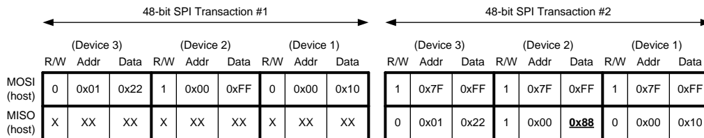
Figure 12. SPI Daisy-Chain Read and Write Example
