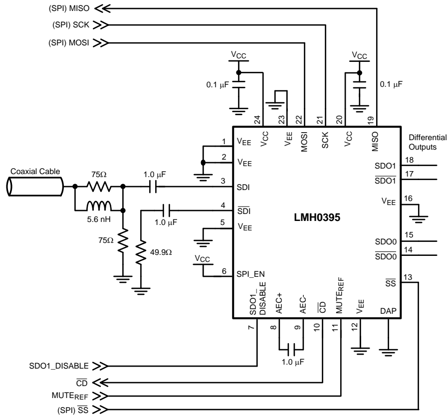
Figure 15. Application Circuit (SPI Mode)
