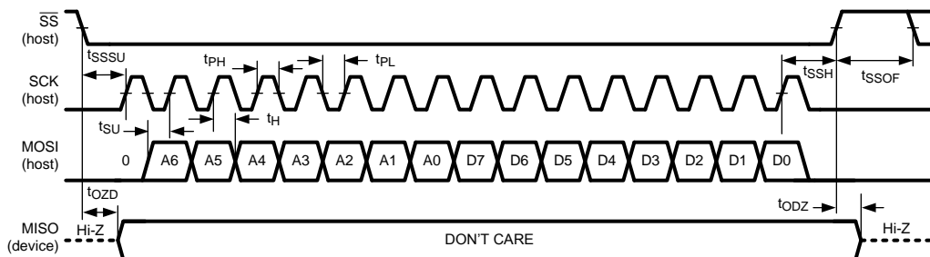
Figure 4. SPI Write
