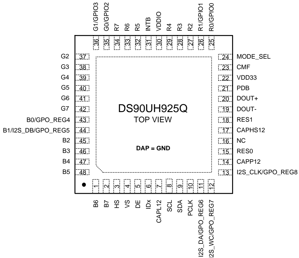
Figure 2. DS90UH925Q — Top View
