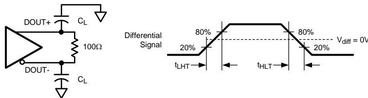
Figure 7. Serializer CML Output Load and Transition Time
