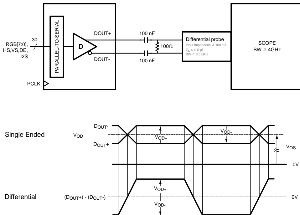
Figure 4. Serializer VOD DC Output
