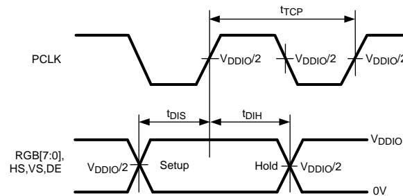
Figure 8. Serializer Setup and Hold Times
