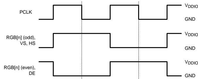
Figure 5. Checkboard Data Pattern
