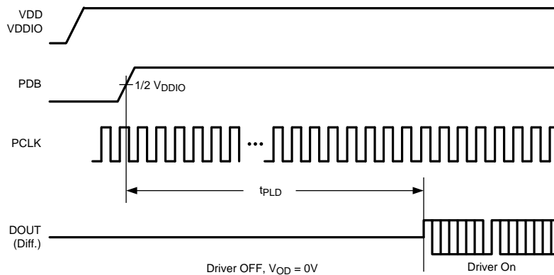
Figure 9. Serializer Lock Time
