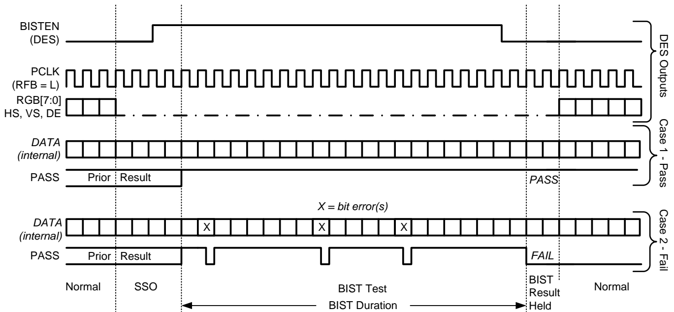
Figure 19. BIST Waveforms
