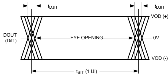
Figure 10. Serializer CML Output Jitter
