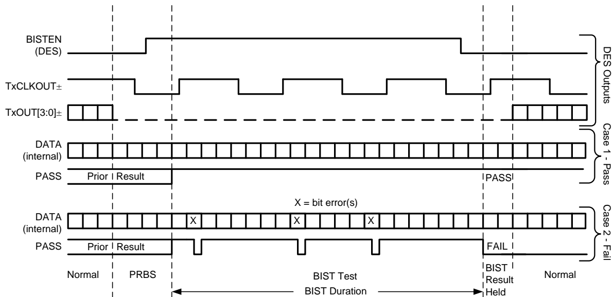
Figure 23. BIST Waveforms
