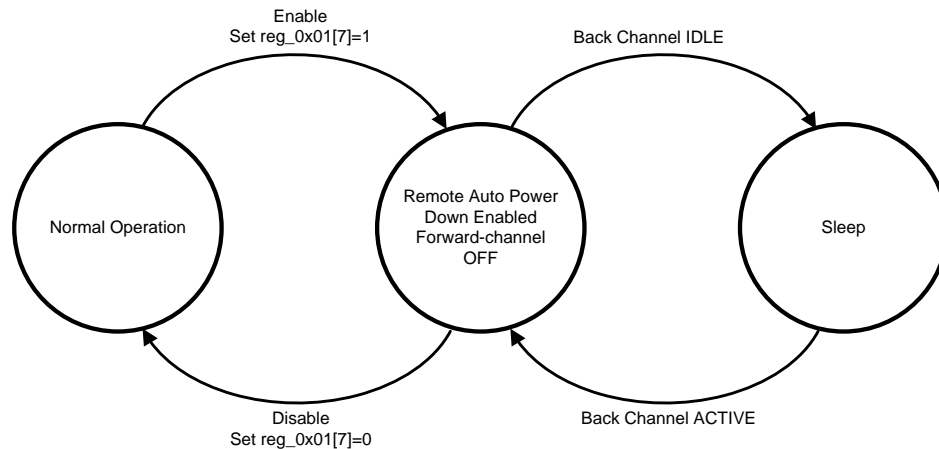
Figure 15. Remote Auto Power Down Sleep/Wake Cycle
