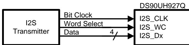
Figure 16. I2S Connection Diagram
