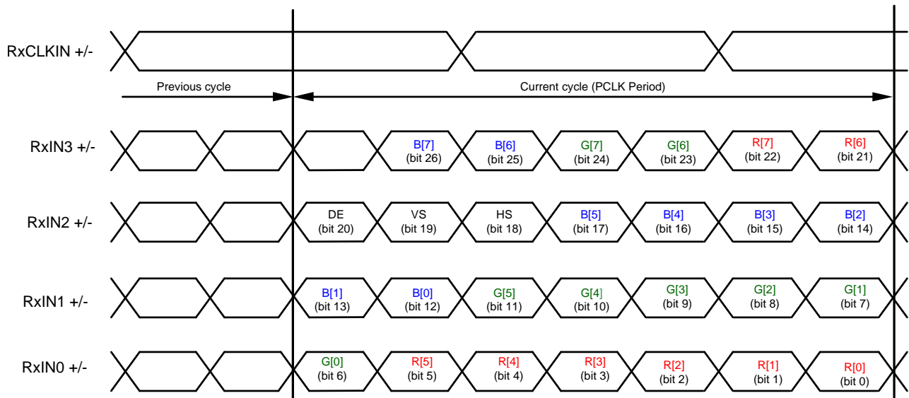
Figure 14. FPD-Link Mapping: MSBs on RxIN3 (MAPSEL=H)
