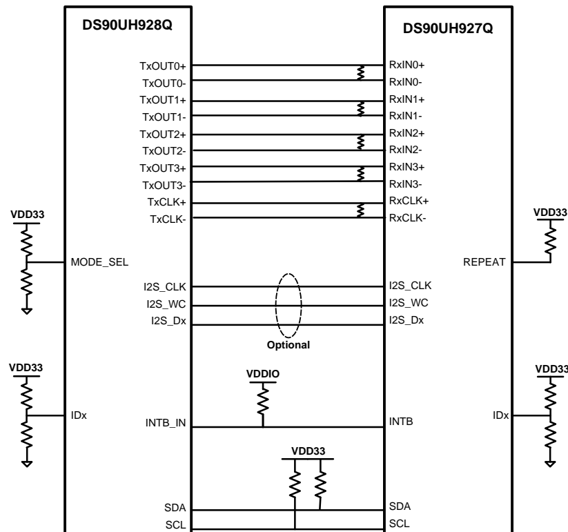
Figure 20. HDCP Repeater Connection Diagram
