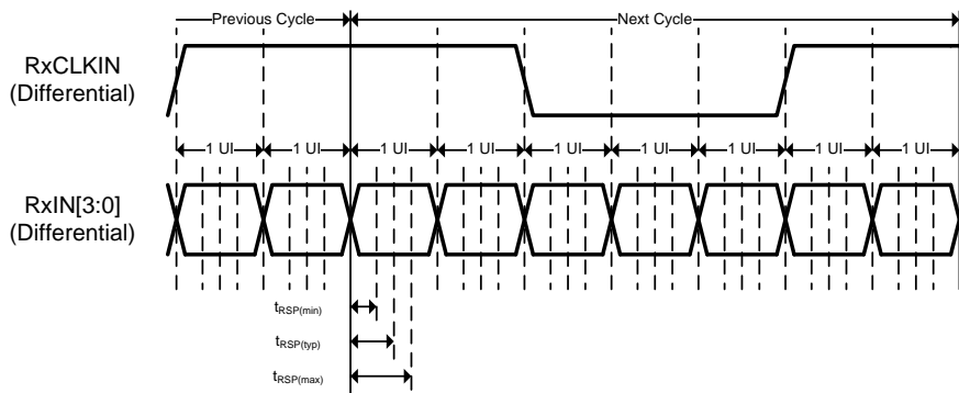
Figure 5. FPD-Link Input Strobe Position
