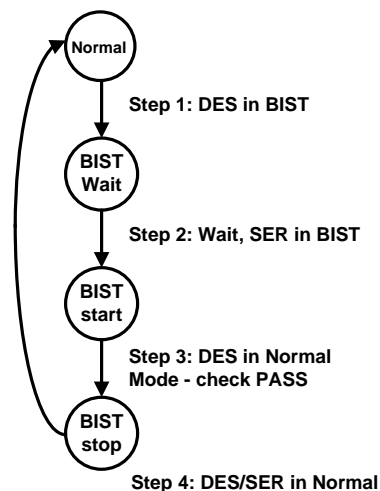
Figure 22. BIST Mode Flow Diagram
