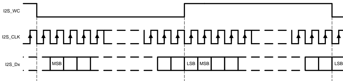
Figure 17. I2S Frame Timing Diagram
