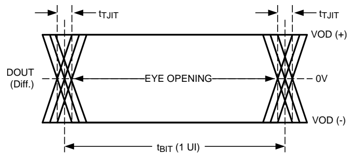
Figure 8. CML Serializer Output Jitter
