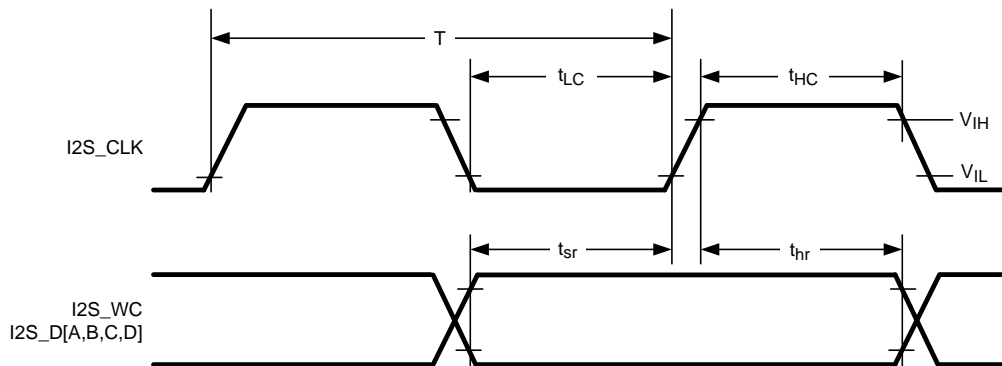
Figure 11. I2S Timing Diagram
