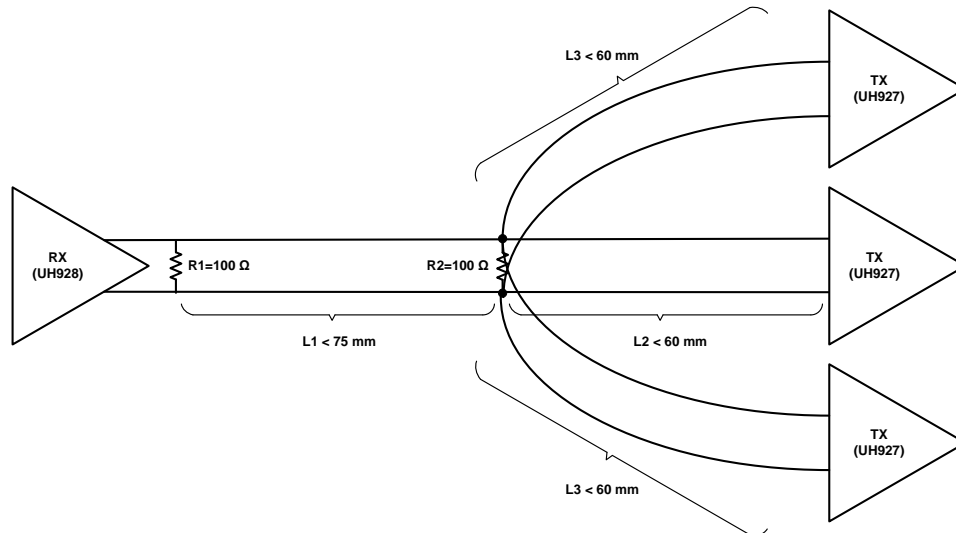
Figure 21. FPD-Link Fan-Out Electrical Requirements
