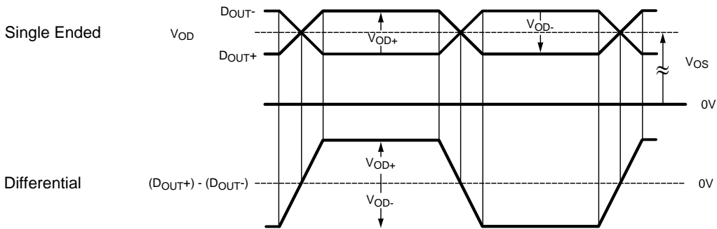
Figure 3. Serializer V_{OD} DC Output
