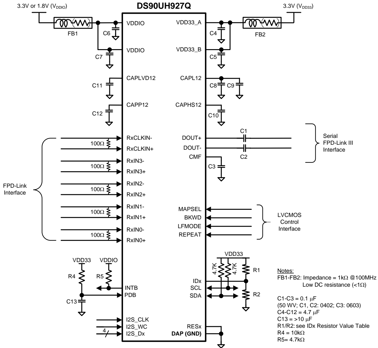
Figure 28. Typical Connection Diagram
