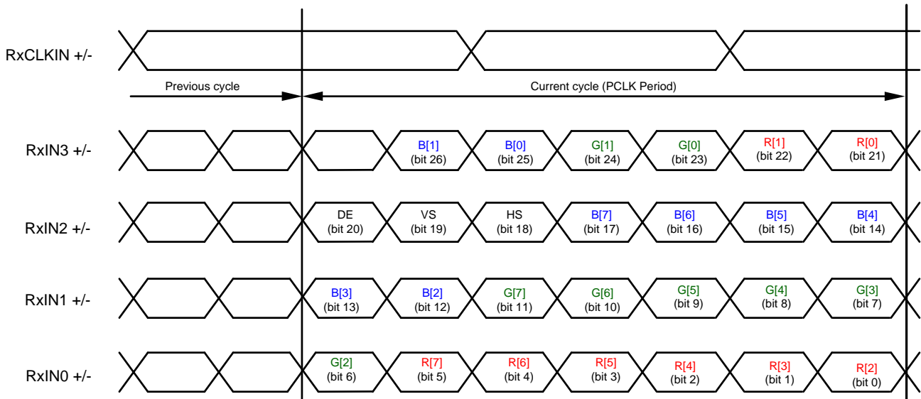
Figure 13. FPD-Link Mapping: LSBs on RxIN3 (MAPSEL=L)
