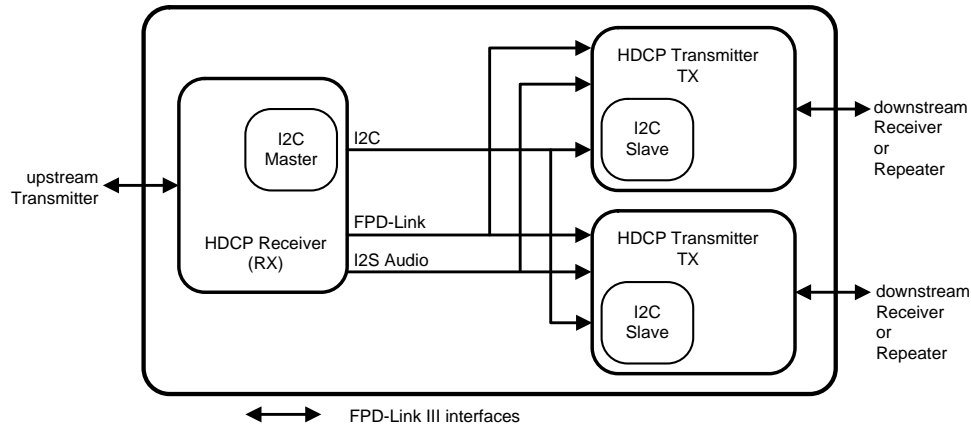
Figure 19. HDCP 1:2 Repeater Configuration
