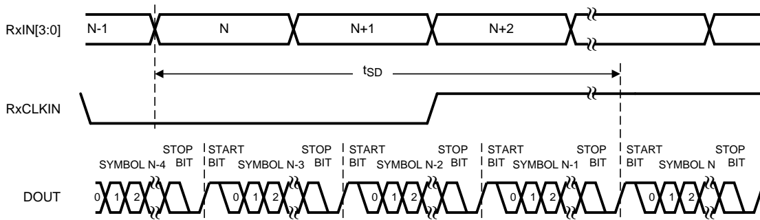
Figure 7. Latency Delay
