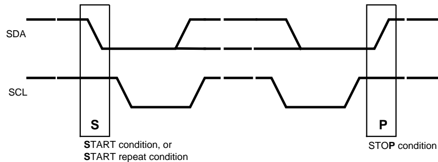
Figure 25. START and STOP Conditions
