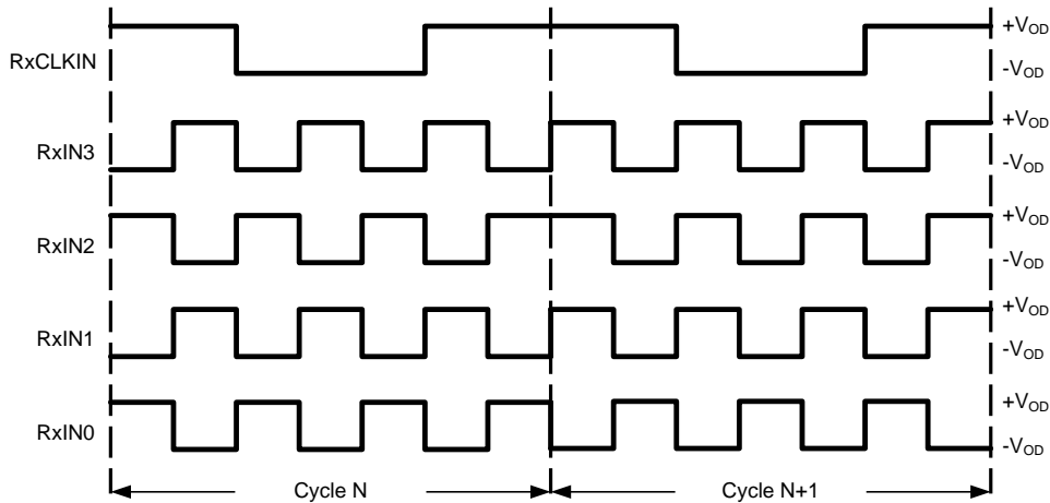
Figure 9. Checkerboard Data Pattern
