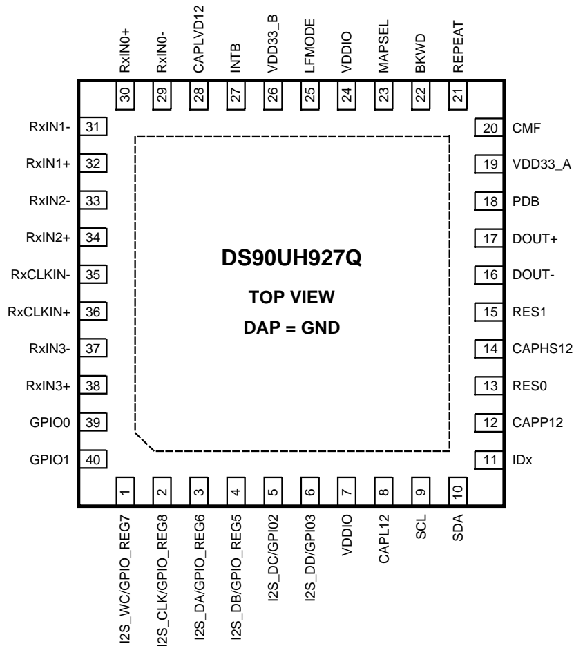
Figure 1. DS90UH927Q — Top View See Package Number RTA-40
