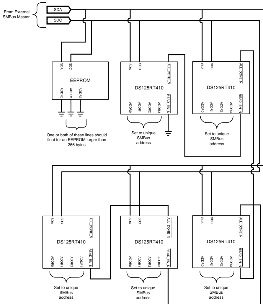
Figure 3. Connection Diagram for Multiple DS125RT410s in SMBus Master Mode
