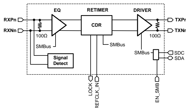
Figure 1. DS125RT410 Data Path Block Diagram — One of Four Channels
