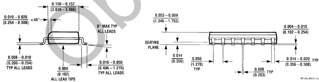
14-Lead Small Outline Molded Package (M) Order Number DM7406M NS Package Number M14A
