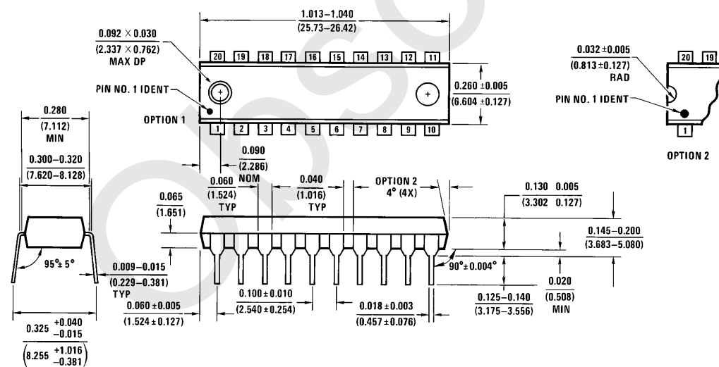
Order Number DM74LS273N NS Package Number N20A
