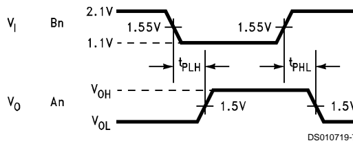
FIGURE 5. Receiver: Bn to An
