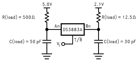
FIGURE 8. T/\bar{R} to An, T/\bar{R} to Bn
