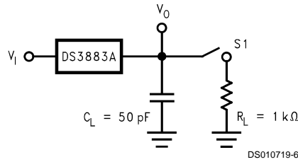
FIGURE 3. Driver: CD to Bn
