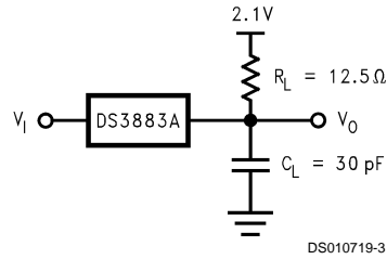
FIGURE 1. Driver Propagation Delay Set-Up
