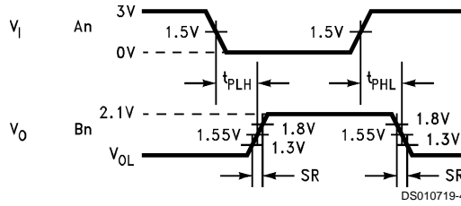
FIGURE 2. Driver: An to Bn, SR
