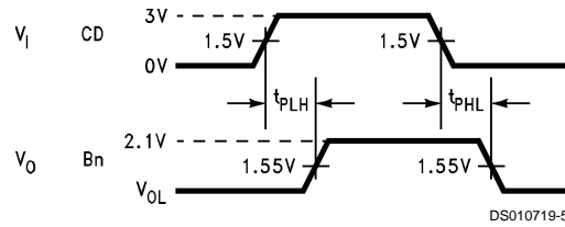
FIGURE 3. Driver: CD to Bn
