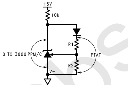
FIGURE 8. Diode in Series with R1 Causes Voltage Across R1 and R2 to be Proportional to Absolute Temperature (PTAT)
